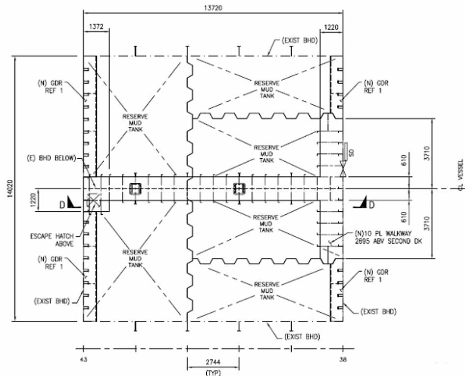
Standard Plan View of Reserve Mud Pit
